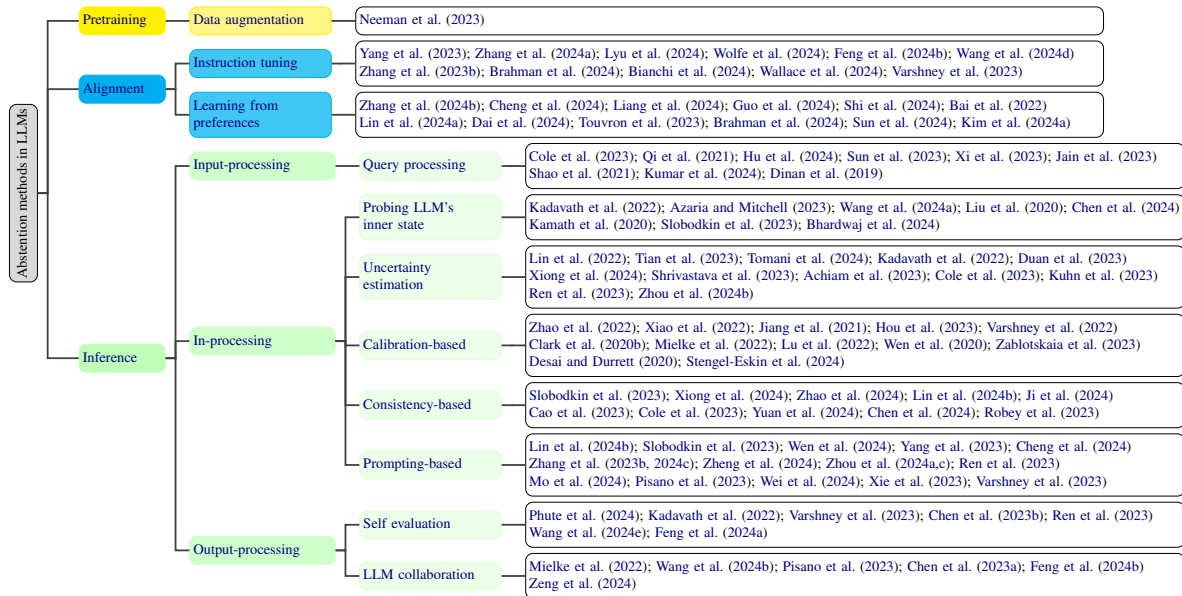
Figure 2: Methods to improve LLM abstinence grouped by pretraining, alignment, and inference stages.
